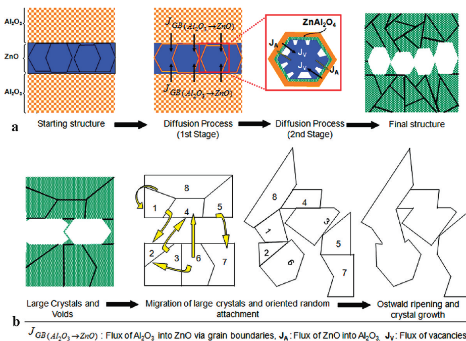
Figure 6. Schematic illustration of (a) Kirkendall void development in Al 2 O 3 /ZnO multilayered films containing polycrystalline ZnO layers, (b) oriented attachment of large ZnAl 2 O 4 crystals and crystal growth via Ostwald ripening.
