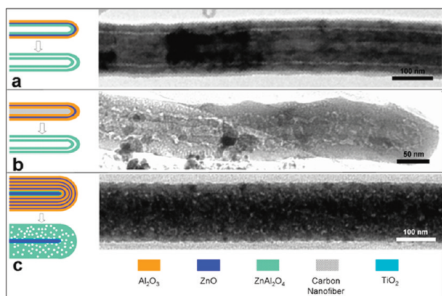
Figure 7. Nanostructures coated with multilayered films illustrated schematically before and after annealing (left) along with a TEM micrograph after annealing (right): (a) ZnAl 2 O 4 nanotube coated with a single pair of ZnO and Al 2 O 3 annealed at 700 °C. (b) Carbon nanofiber coated with a multilayered film with three alternating layers of Al 2 O 3 and ZnO annealed at 700 °C. (c) ZnO nanowire coated with a multilayered film with nine alternating layers of Al 2 O 3 and ZnO annealed at 800 °C.
